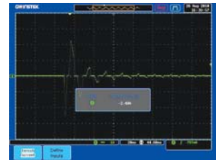
In-rush Current
